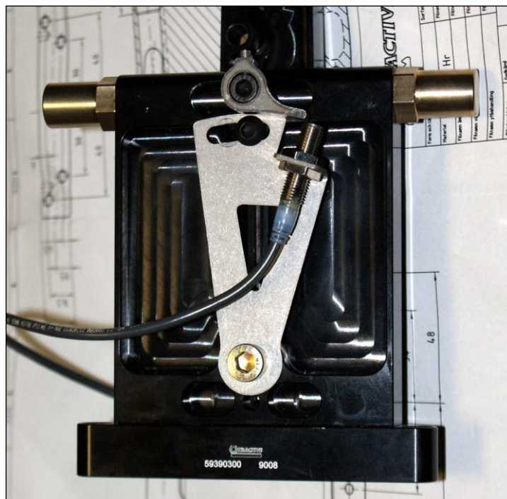
Tractive gearlever with mounting bracket 40-110-4 and sensor 30-521-9
